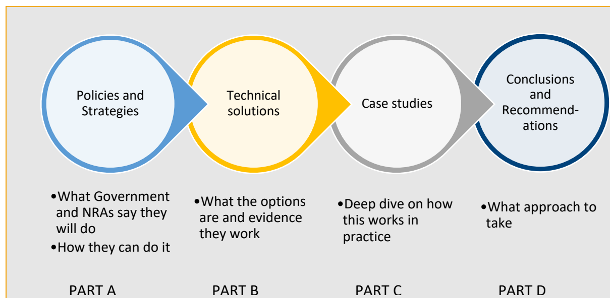
Figure 5. Document structure
