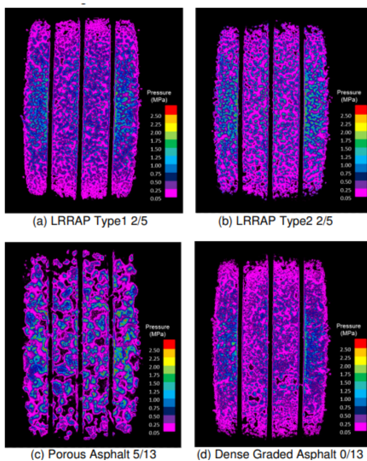
Figure 13. Contact pressures between the tyre and pavement surfaces from Ishigaki et al. 133
