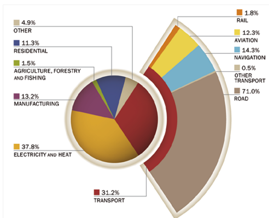
Figure 1. CO 2 emissions from fuel combustion by sector
